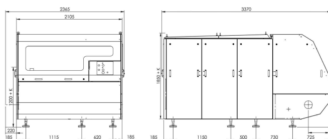
Overall dimensions (mm)
