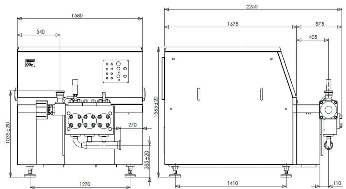
Overall dimensions (mm)
